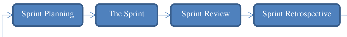
Figur 2 Sprint Cycle
